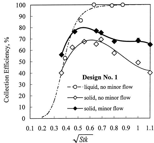
FIG. 4 Particle collection efficiency curve, design no. 1, S/W = 4.0 .
