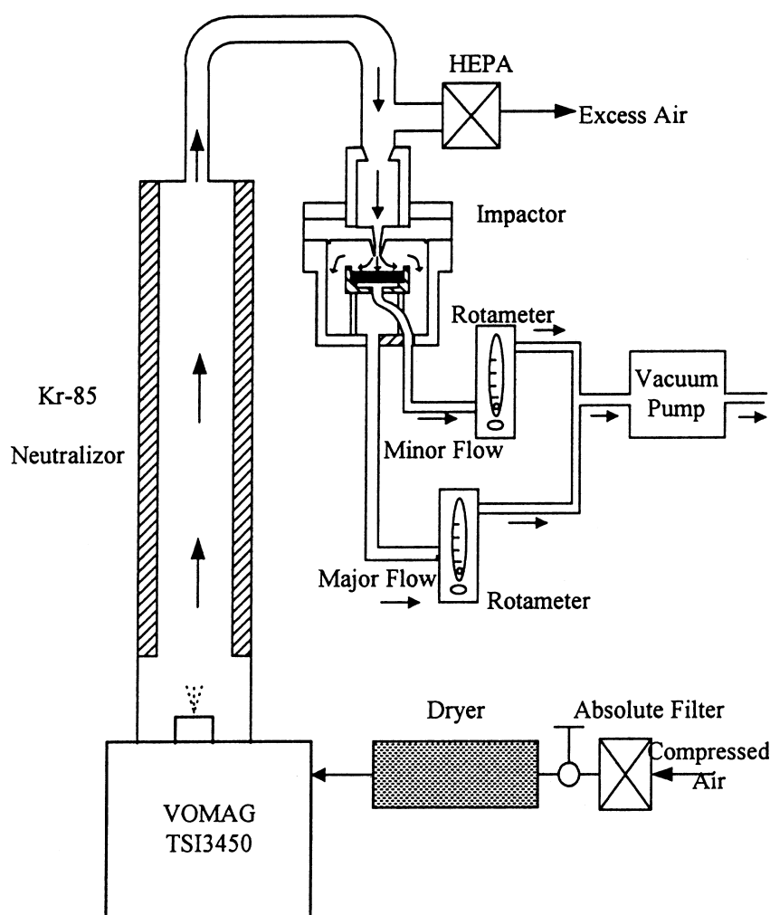
FIG. 2 The experimental setup.
