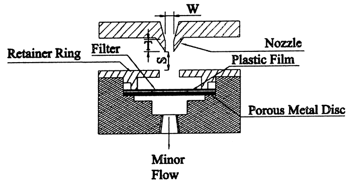
(c) Design No. 3
