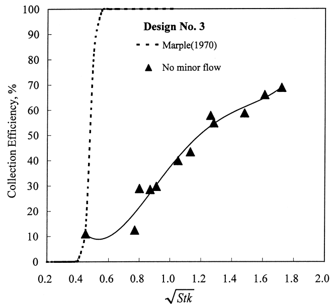
FIG. 9 Particle collection efficiency curve, design no. 3.
