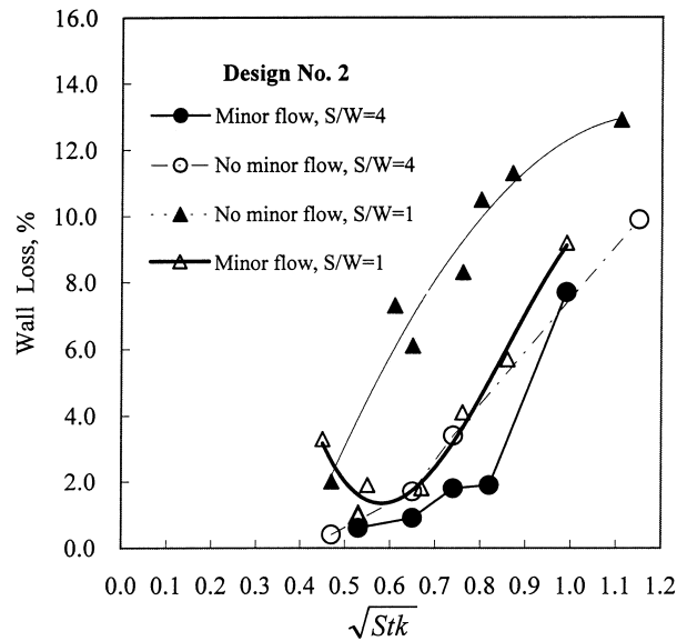
FIG. 8 Particle wall loss, design no. 2.
