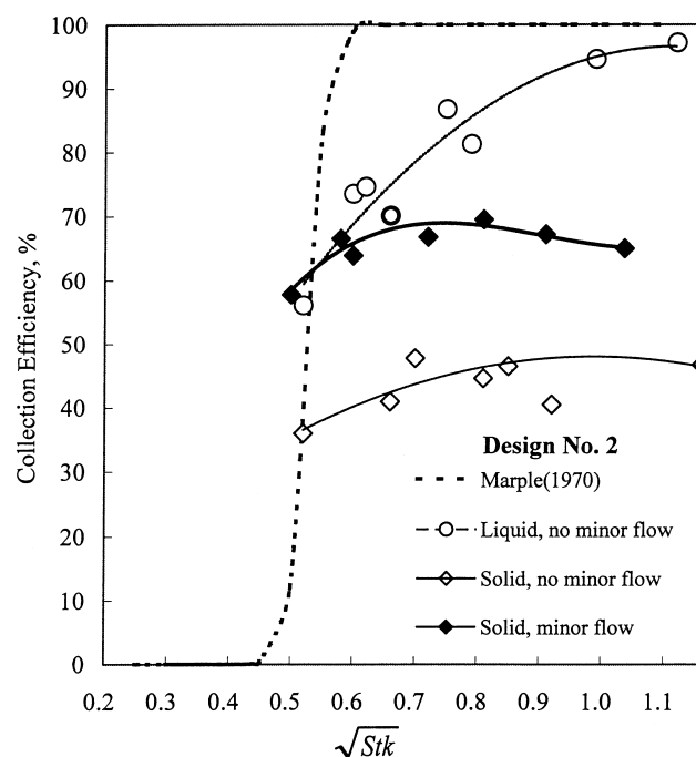
FIG. 6 Particle collection efficiency curve, design no. 2, S/W = 1.0 .
