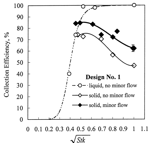
FIG. 3 Particle collection efficiency curve, design no. 1, S/W = 1.0 .
