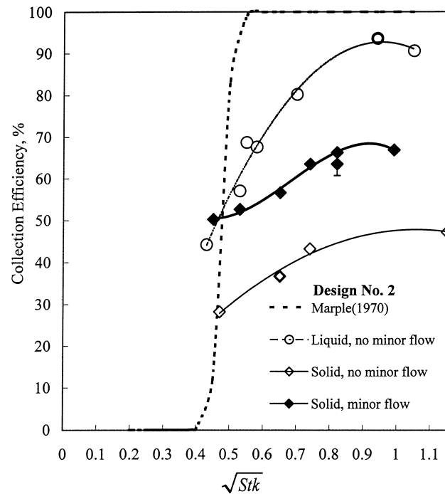
FIG. 7 Particle collection efficiency curve, design no. 2, S/W = 4.0 .
