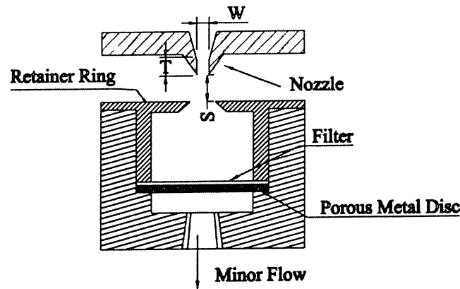
FIG. 1 Three different impactor designs.
