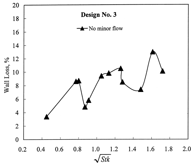
FIG. 10 Particle wall loss, design no. 3.
