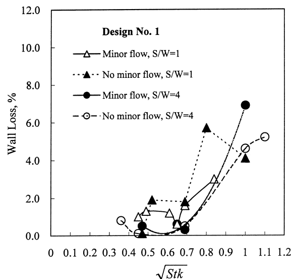
FIG. 5 Particle wall loss, design no. 1.
